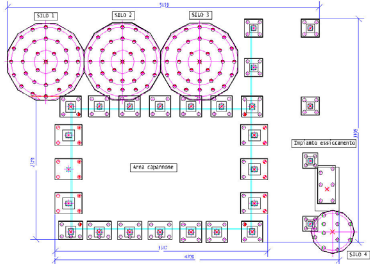
▲ Colonne in Ghiaia Vibrocompattate Cementate CGVC
